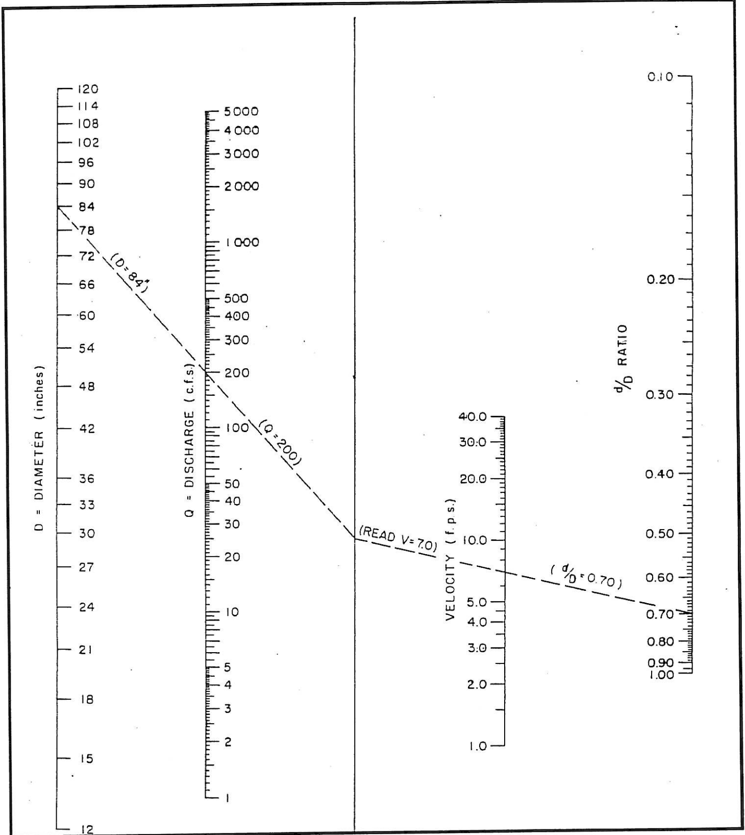
Exhibit 900-18 Velocity in Pipe Conduits
