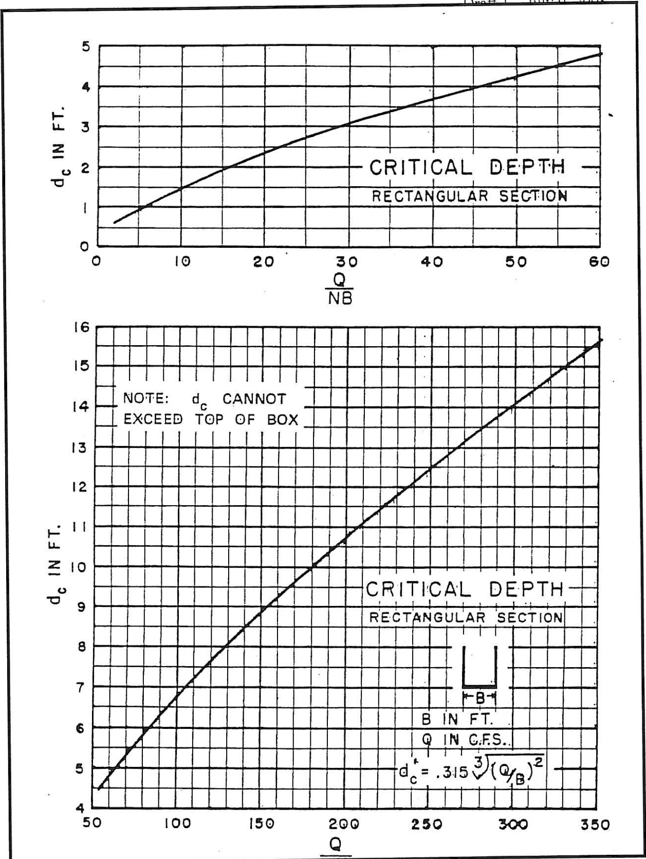
Exhibit 900-5 Critical Depth Rectangular Section Source: Arkansas Highway and Transportation Department Drainage Manual
