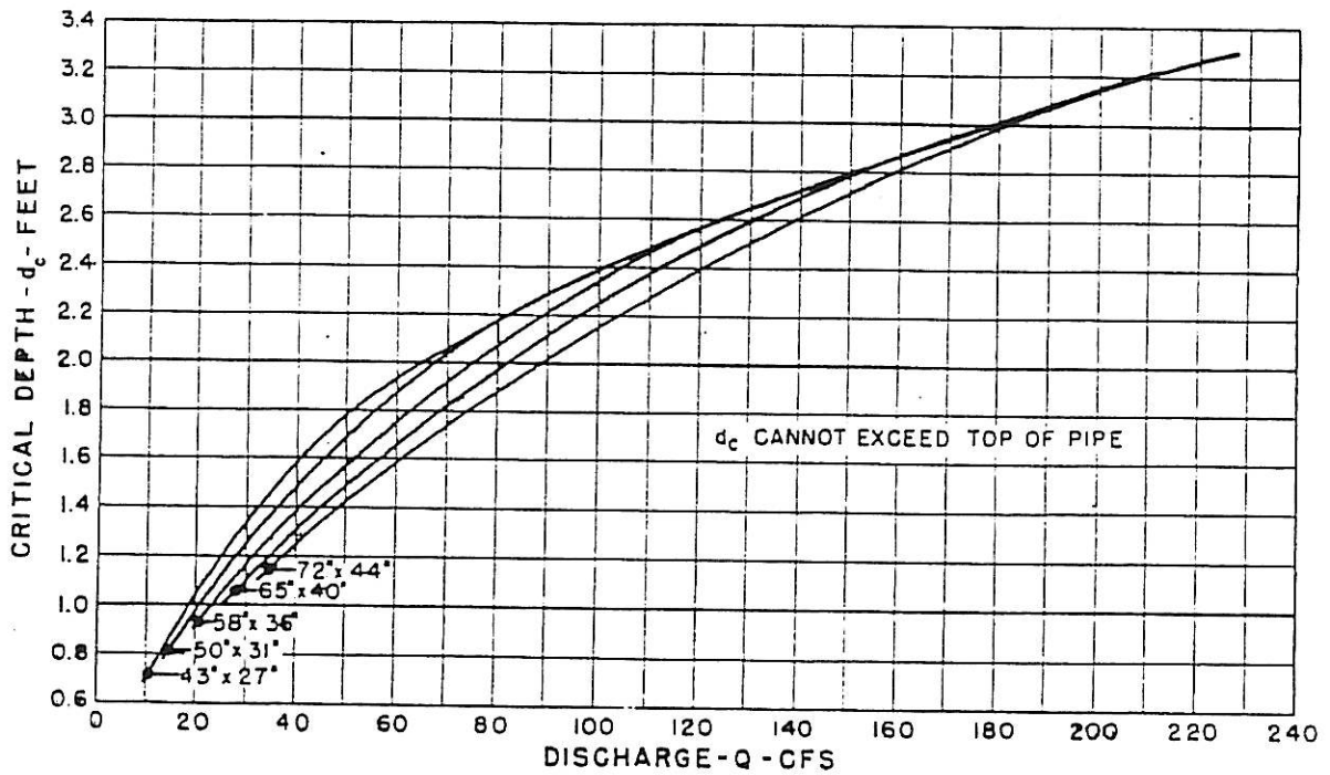
Exhibit 900-21 Critical Depth Standard C.M. Pipe-Arch Source: Arkansas Highway and Transportation Department Drainage Manual
