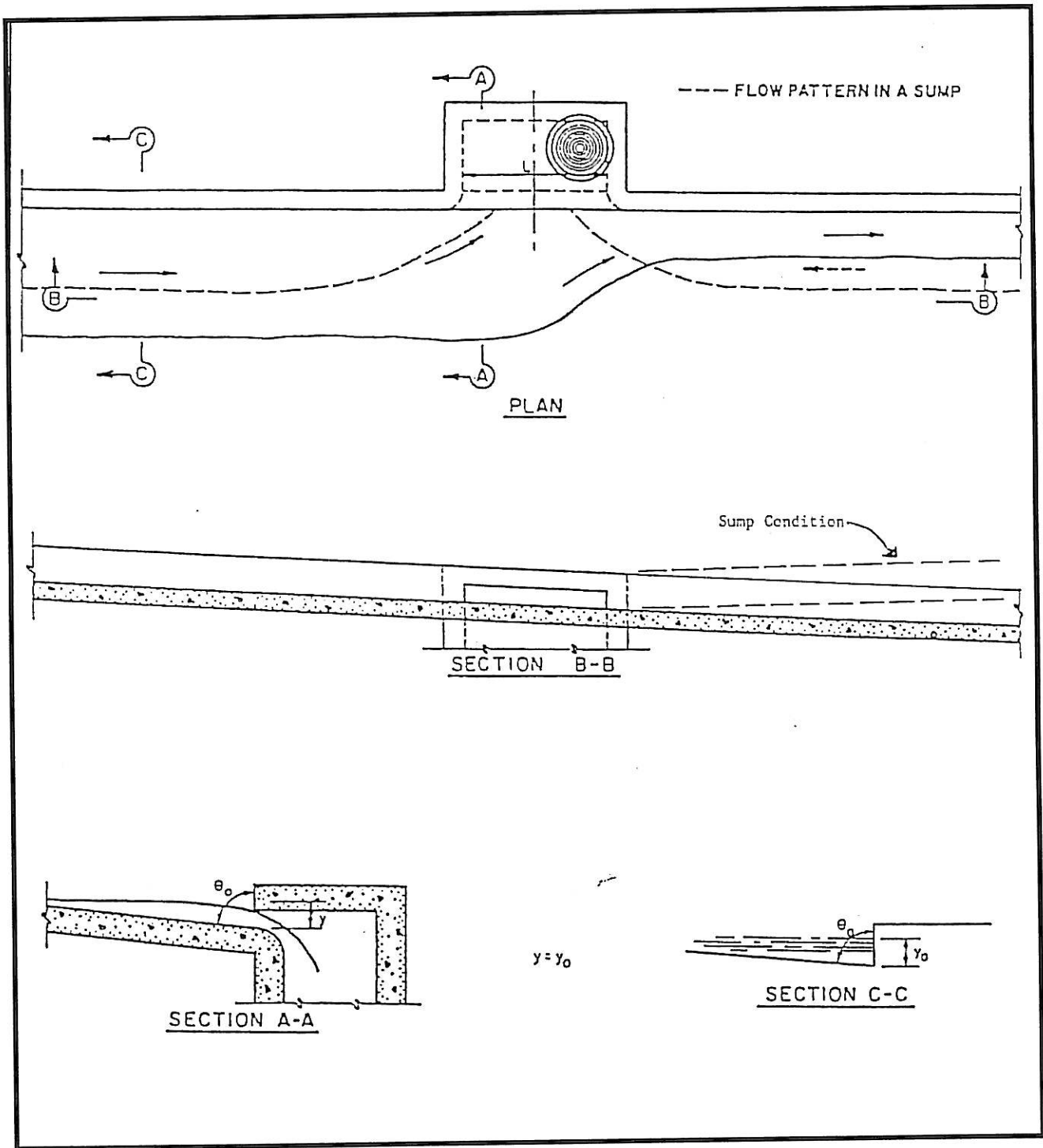
Exhibit 800-5 Undepressed Curb Opening Inlet Type A-1 & B-1 (Recessed) Source: (City of Little Rock Stormwater Drainage Manual)
