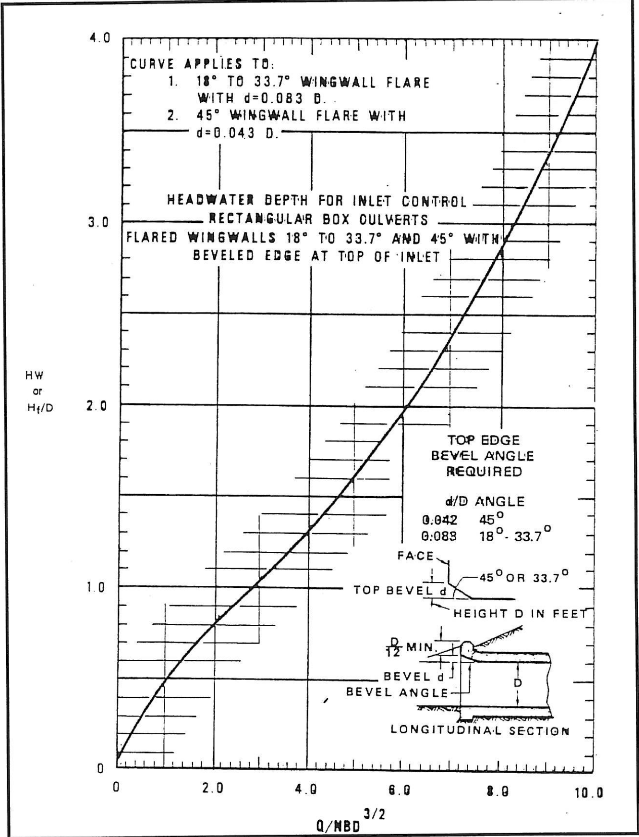
Exhibit 900-8 Headwater Depth for Inlet Control Rectangular Box Culverts Flared Wingwalls 18° to 33.7° to 45° with Beveled Edge at Top of Inlet Source: Arkansas Highway and Transportation Department Drainage Manual
