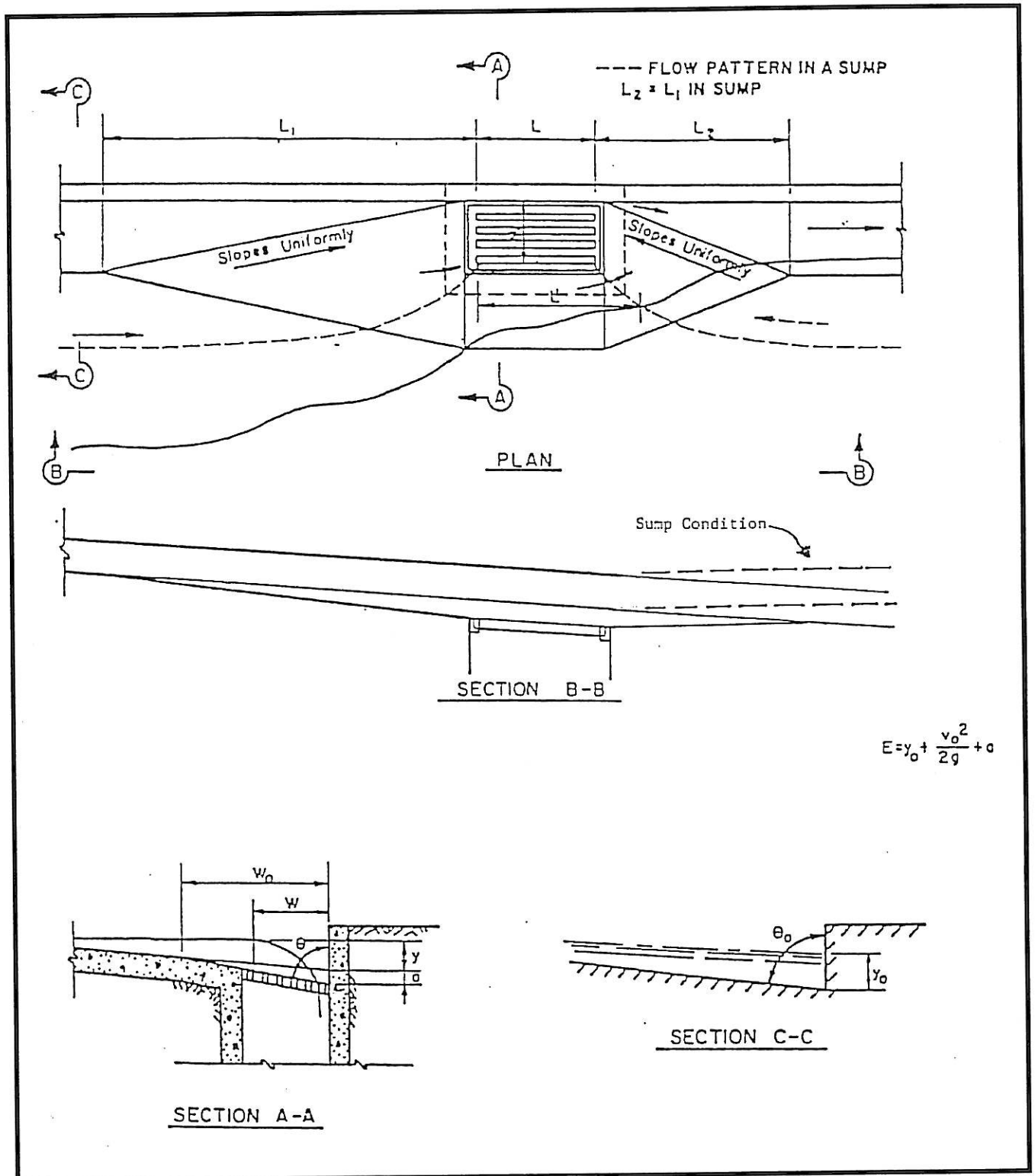
Exhibit 800-2 Depressed Grate Inlet (Type A-2 and Type C-2) Source: (City of Little Rock Stormwater Drainage Manual)
