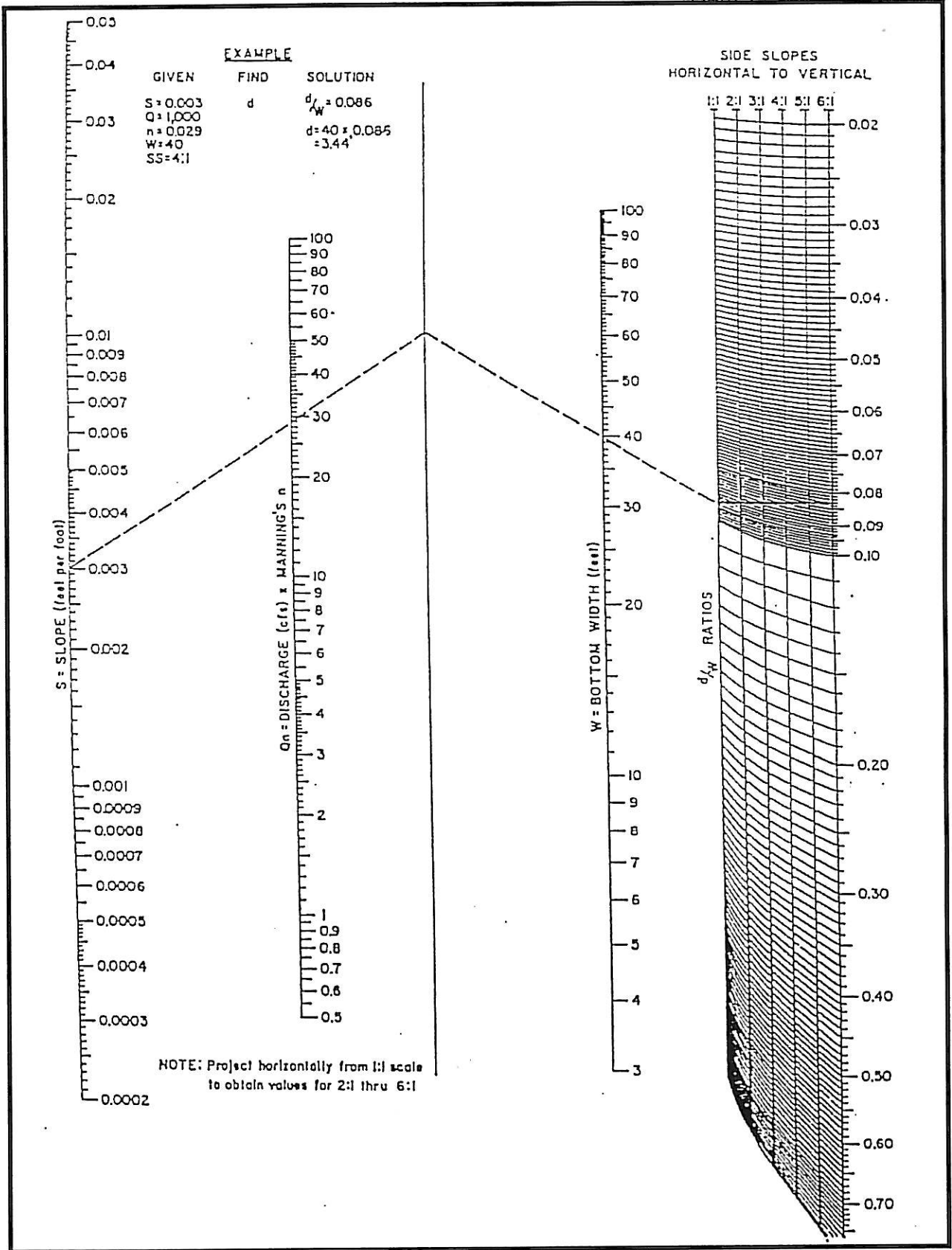
Exhibit 500-4 Uniform Flow for Trapezoidal Channels (Source: Arkansas Highway and Transportation Department Drainage Manual)
