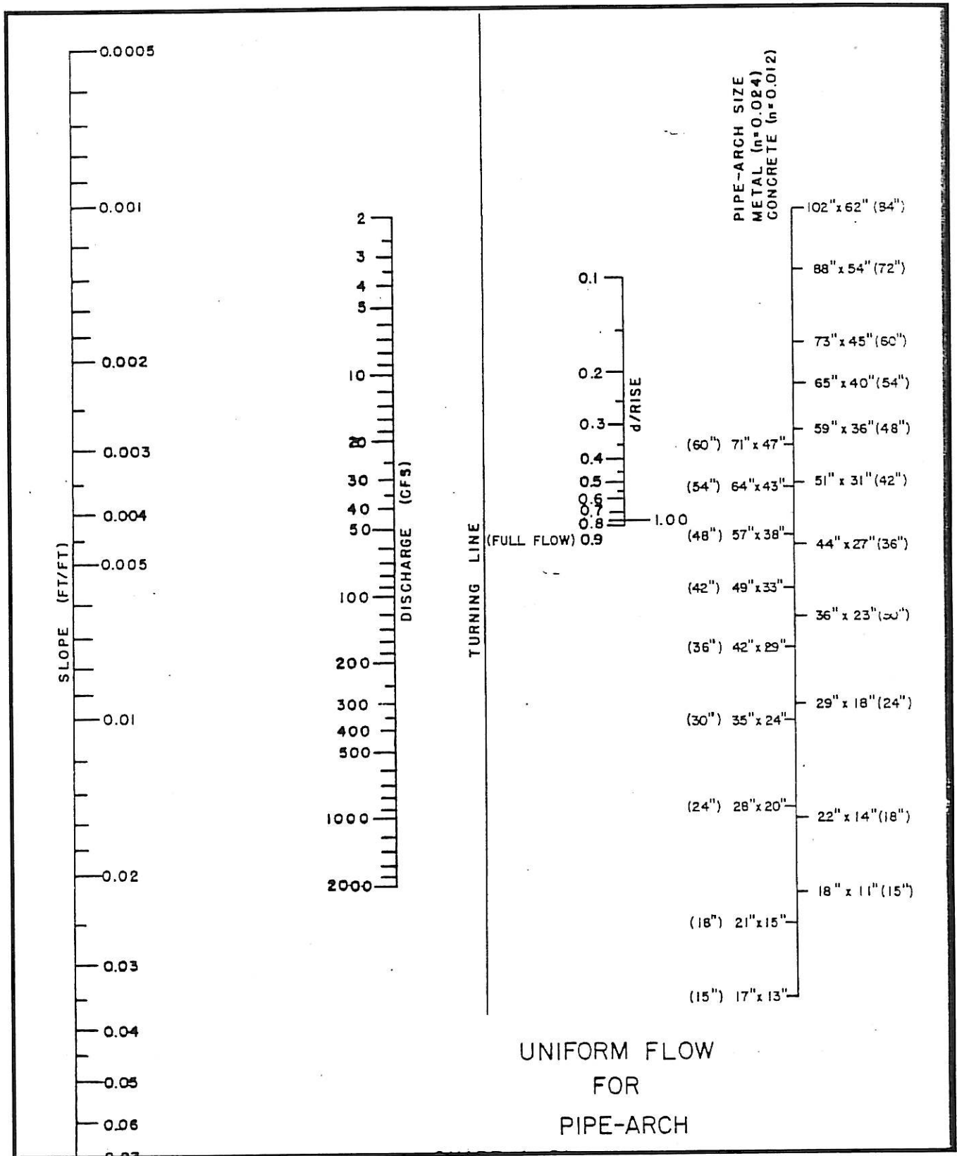
Exhibit 900-24 Uniform Flow for Pipe-Arch Source: Arkansas Highway and Transportation Department Drainage Manual
