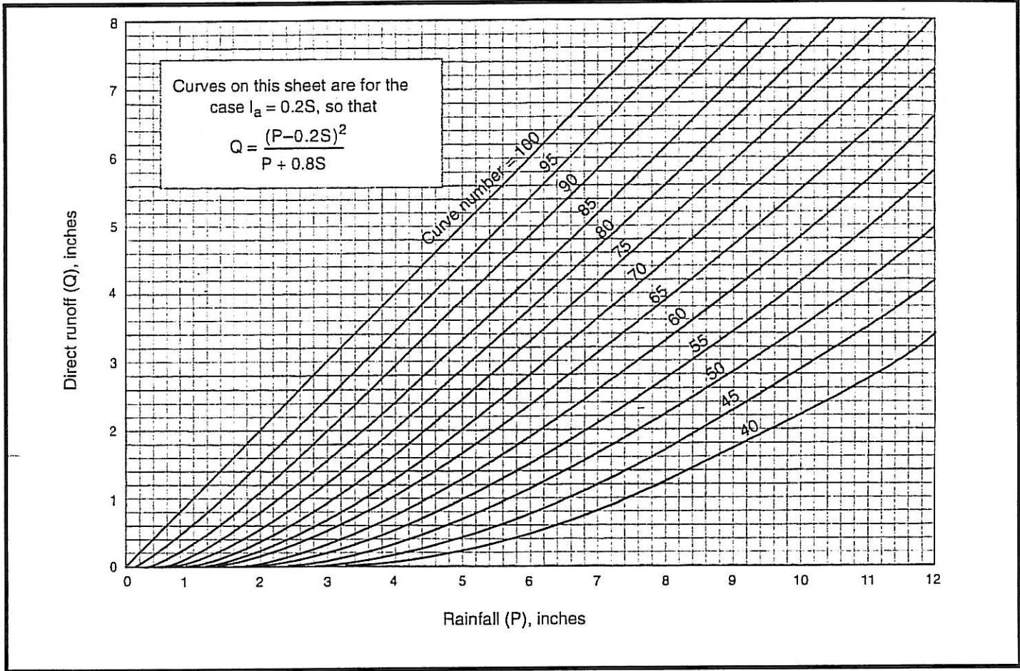
Exhibit 400-5 Solution of Runoff Equation (Source: NRCS (SCS) TR55)
