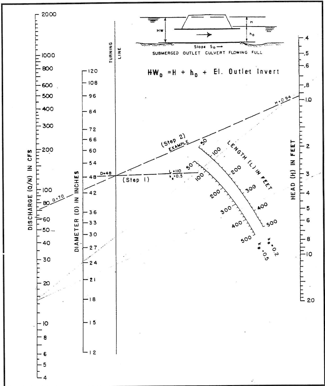
Exhibit 900-12 Head for Concrete Pipe Culverts Flowing Full (n=0.012) Source: Arkansas Highway and Transportation Department Drainage Manual
