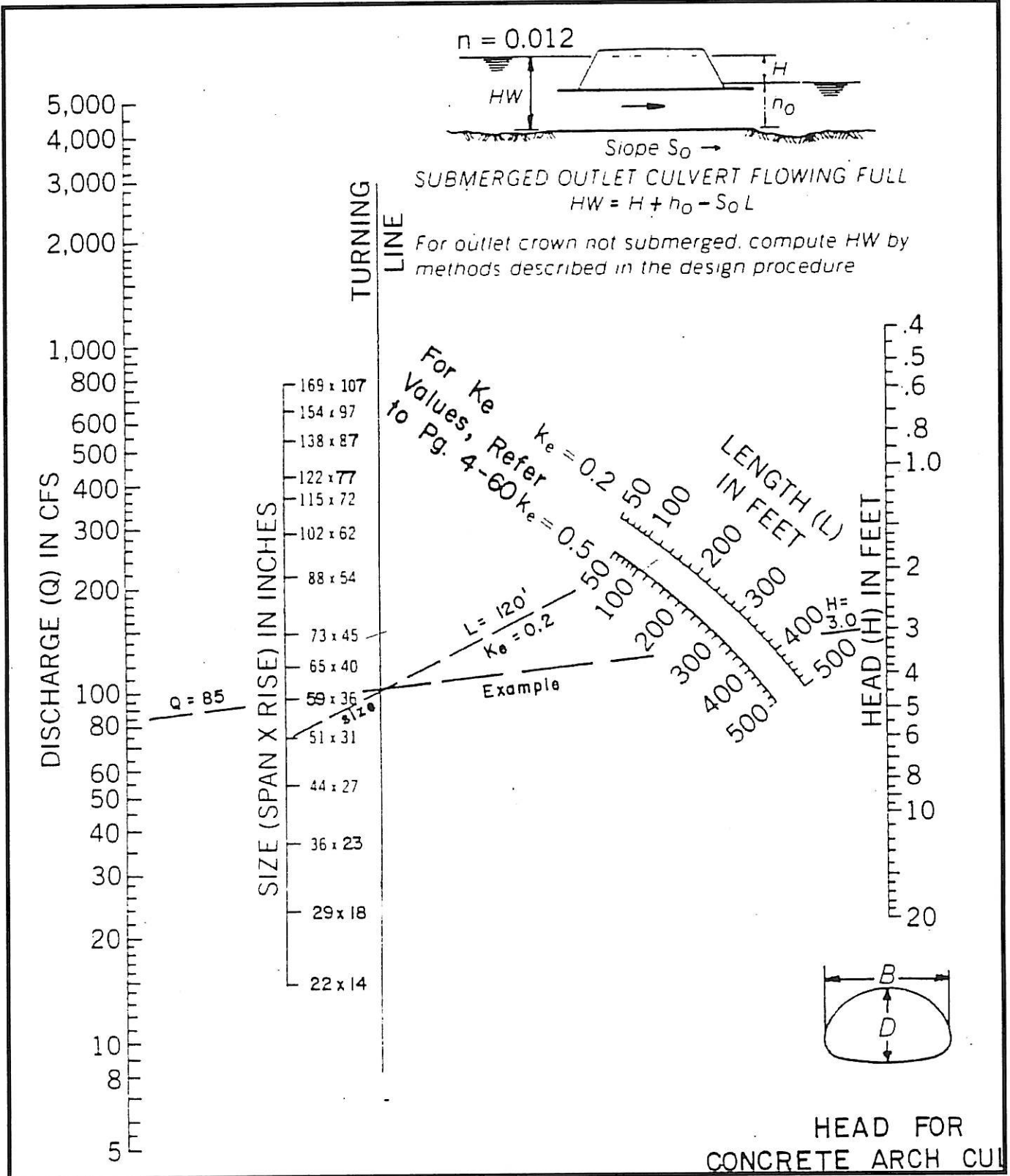
Exhibit 900-19.1 Head for Concrete Arch Culvert Flowing Full ( n=0.012 ) Source: Arkansas Highway and Transportation Department Drainage Manual
