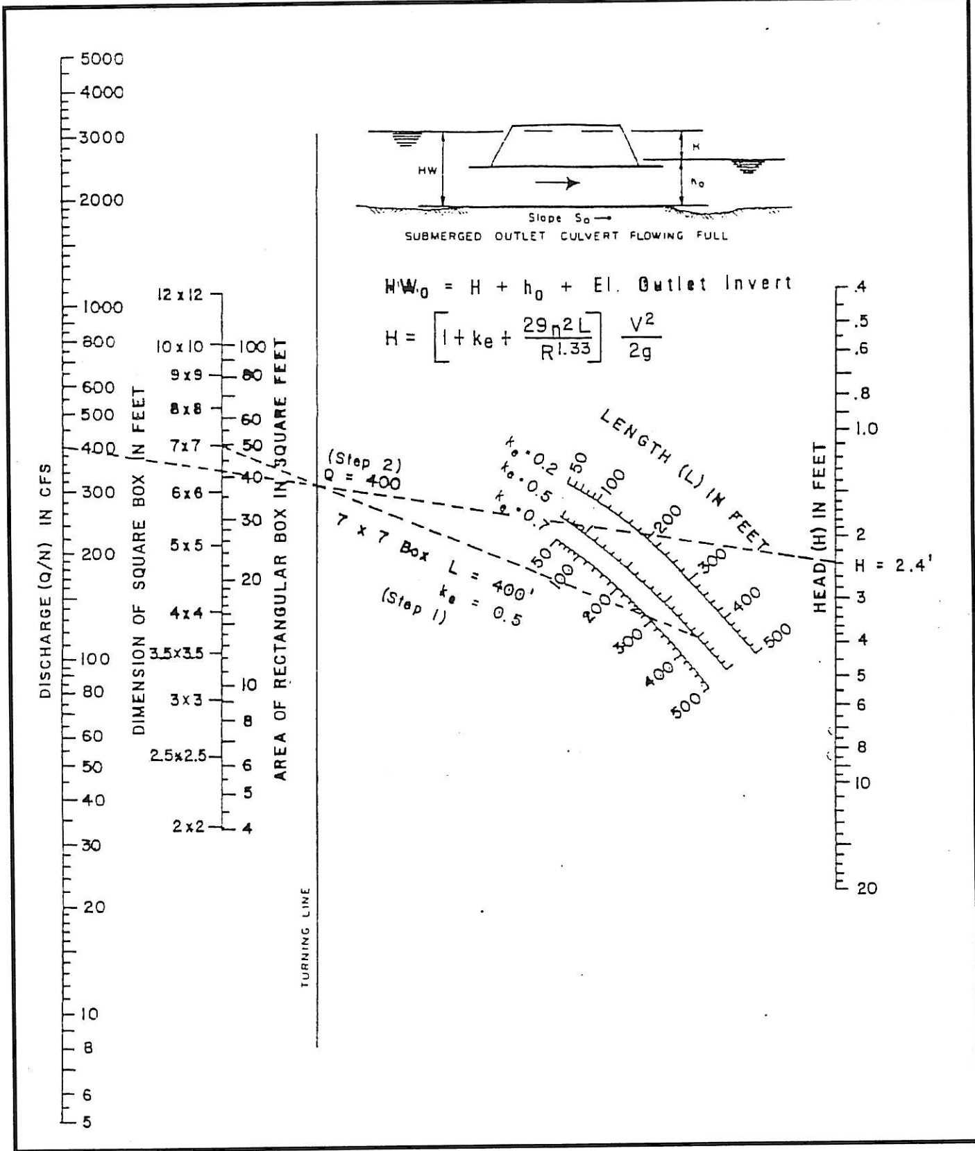
Exhibit 900-4 Head for Concrete Box Culverts Flowing Full (n = 0.012) Source: Arkansas Highway and Transportation Department Drainage Manual
