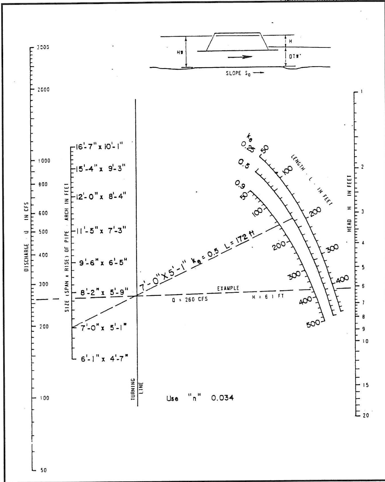
Exhibit 900-20.1 Head for Structural Plate C.M. P. Arch Source: Arkansas Highway and Transportation Department Drainage Manual
