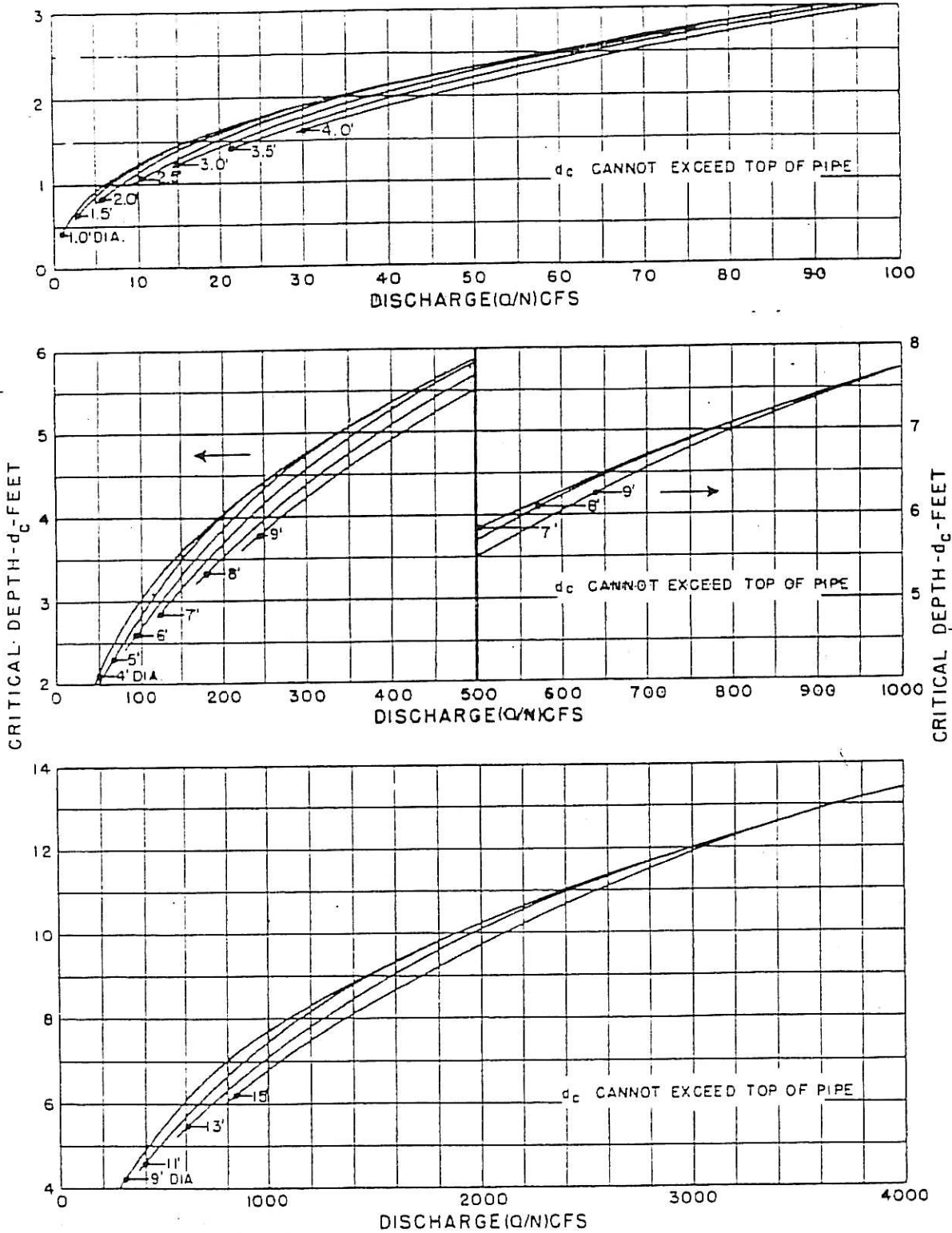
Exhibit 900-14 Critical Depth Circular Pipe Source: Arkansas Highway and Transportation Department Drainage Manual
