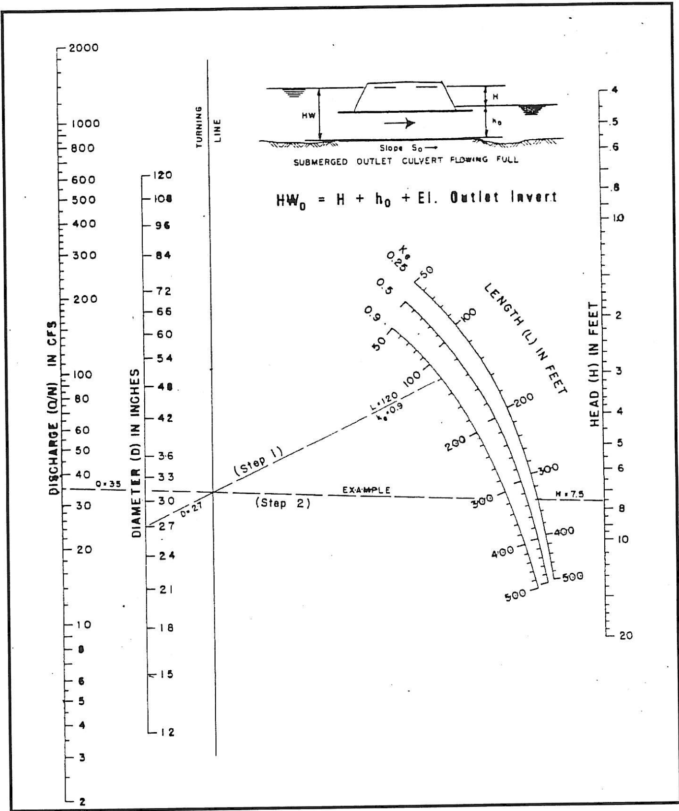
Exhibit 900-13 Head for Standard C.M. Pipe Culverts Flowing Full (n=0.024) Source: Arkansas Highway and Transportation Department Drainage Manual
