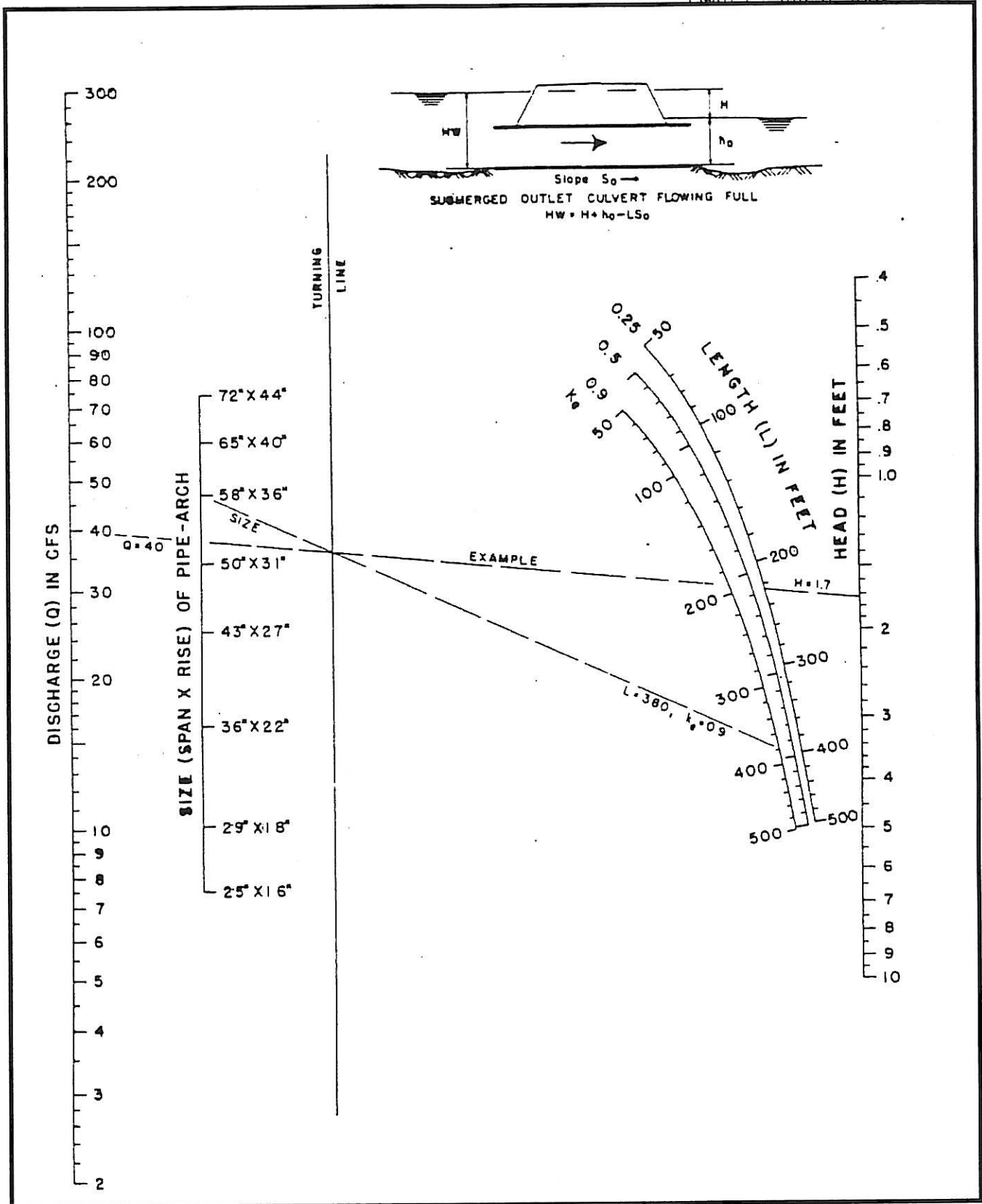
Exhibit 900-20 Head for Standard C.M. Pipe-Arch Culverts Flowing Full ( n = 0.024 ) Source: Arkansas Highway and Transportation Department Drainage Manual
