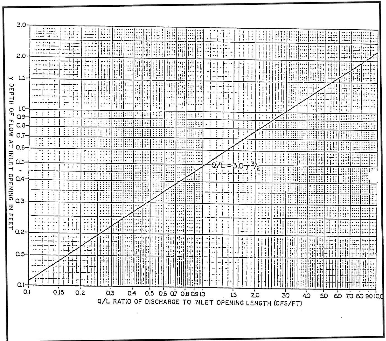
Exhibit 800-8 Inlet Capacity (Type A-1 & A-4) Source: (City of Little Rock Stormwater Drainage Manual)
