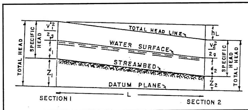
(Source: Arkansas Highway and Transportation Department Drainage Manual) Figure 500-1 Water surface profile of channel with uniform flow.
