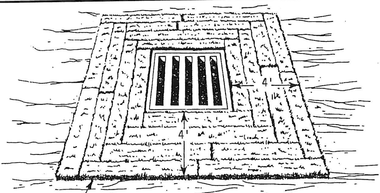
Four 1-foot Wide Strips of Sod on Each Side of the Drop Inlet
