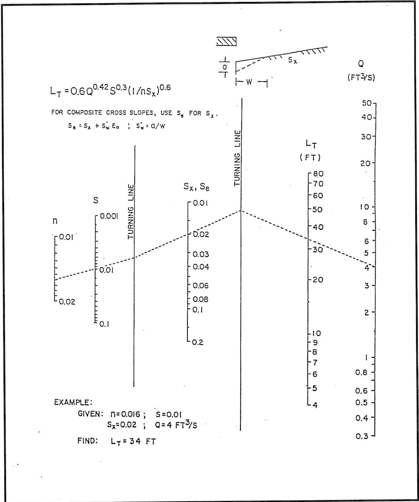
Exhibit 800-10 Curb-Opening and Slotted Drain Inlet Length for Total Interception
