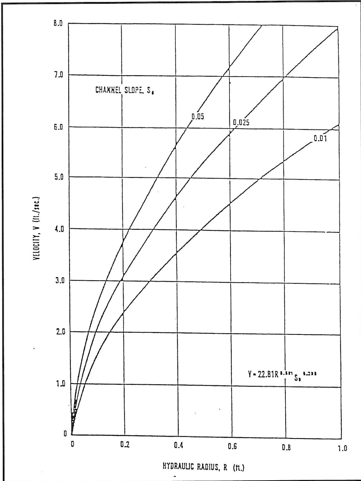
Exhibit 500-3 Flow Velocity for Unlined Channels (Bare Soil) (Source: Arkansas Highway and Transportation Department Drainage Manual)
