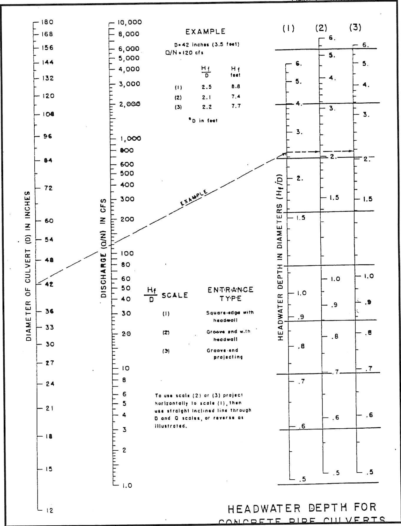
Exhibit 900-15 Headwater Depth for Concrete Pipe Culverts with Inlet Control Source: Arkansas Highway and Transportation Department Drainage Manual
