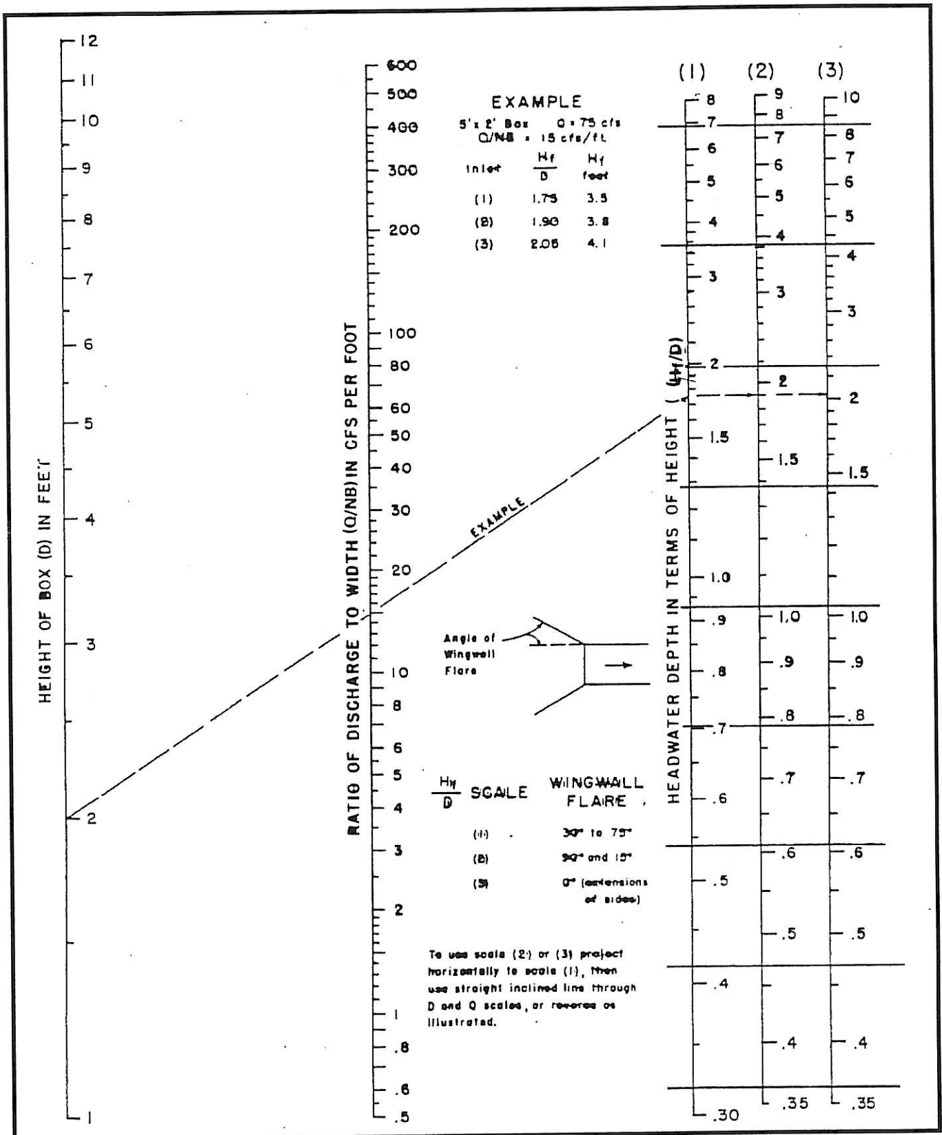
Exhibit 900-7 Headwater Depth for Box Culverts with Inlet Control Source: Arkansas Highway and Transportation Department Drainage Manual
